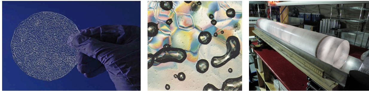
Figure 7: Ice cores have been drilled in different locations in Antarctica ( top left ) ( inactive link as of 10/02/2020 ) using drilling devices like the one depicted here ( top center ). Air gets trapped in the ice through compaction of snow and firn ( top right ). These air bubbles in the ice are visible by eye ( bottom left ) and in the microscope ( bottom center ). Sometimes dark ash layers are found in ice cores, which can help to date the ice ( bottom right ).
