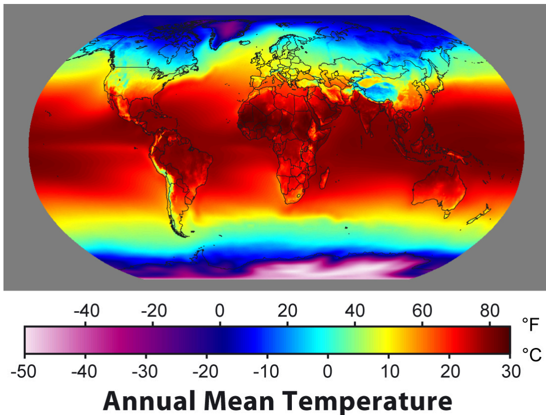
Figure 1: Annual mean surface temperature distribution. From wikimedia.org .
