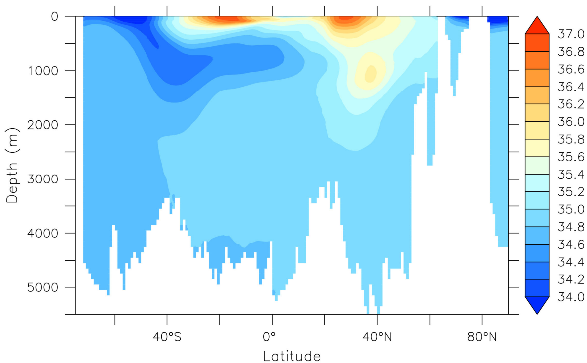
Figure 19: Salinity (in grams salt per kg of sea water) section through the Atlantic ocean at 18^\circ\text{W} as a function of latitude and depth.
