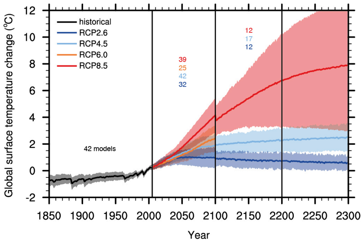
Figure 3. Global average surface temperature projections relative to 1886-2005. Shading indicates the 5 and 95% range and the line is the multi model mean. The black line with the grey shading represents historical simulations including variations in volcanic forcing. Since volcanic forcing is impossible to predict for the future, changes in natural radiative forcings are not considered in the projections. The number of climate models used is indicated. Not all models have simulated the full period until year 2300, which leads to a jump in the red line at year 2100. From ipcc.ch .
