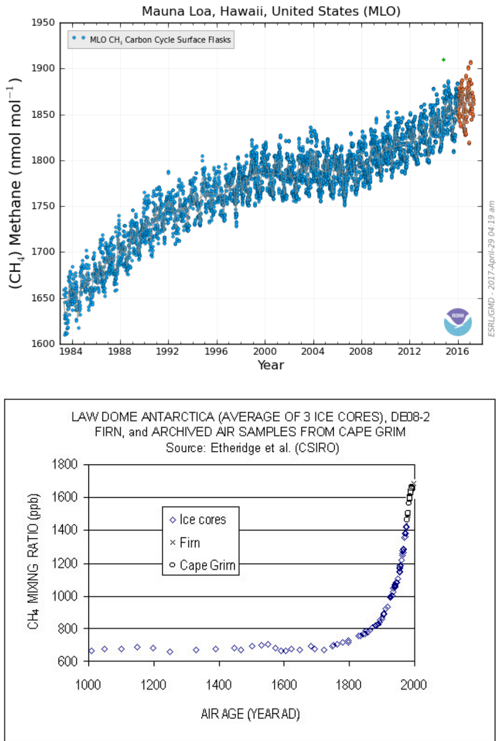
Figure 10: Top : Atmospheric methane concentrations as a function of time. Top: Recent air measurements from Mauna Loa. Bottom : Ice core, firn, and air measurements from Antarctica. Note that most methane sources are in the northern hemisphere, which leads to higher concentrations there compared with the southern hemisphere.
