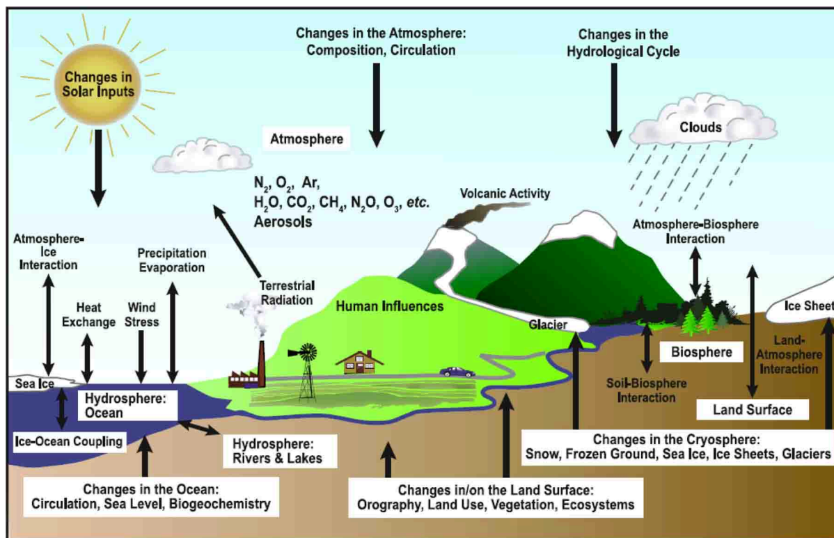
Figure 2: Schematic view of components of the climate system and processes involved in their interactions. From Le Treut et al. (2007). https://www.ncdc.noaa.gov/cagTreut et al. (2007).
