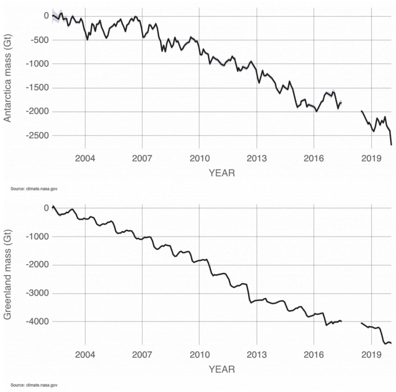
Figure 7: Changes in the Antarctic (top) and Greenland (bottom) ice sheet mass estimated from satellite gravity measurements. From nasa.gov .
