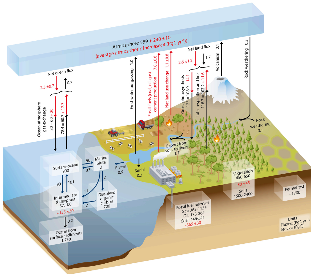
Figure 1: The Carbon Cycle. Numbers in boxes represent reservoir mass, also called carbon stocks, inventories, or storage in PgC (1 Pg = 10^{15} g = 1 Gt). 2.1 PgC = 1 ppm atmospheric CO 2 . Numbers next to arrows indicate fluxes in PgC/yr. Black numbers and arrows represent estimates of the natural (pre-industrial) carbon cycle. Red numbers and arrows indicate estimates of anthropogenic effects for 2000-2009. From Ciais et al. (2013). Image from ipcc.ch . See additional material at the end of this chapter for a figure showing the sizes of the reservoirs and fluxes in proportion to the size of the boxes and arrows.
